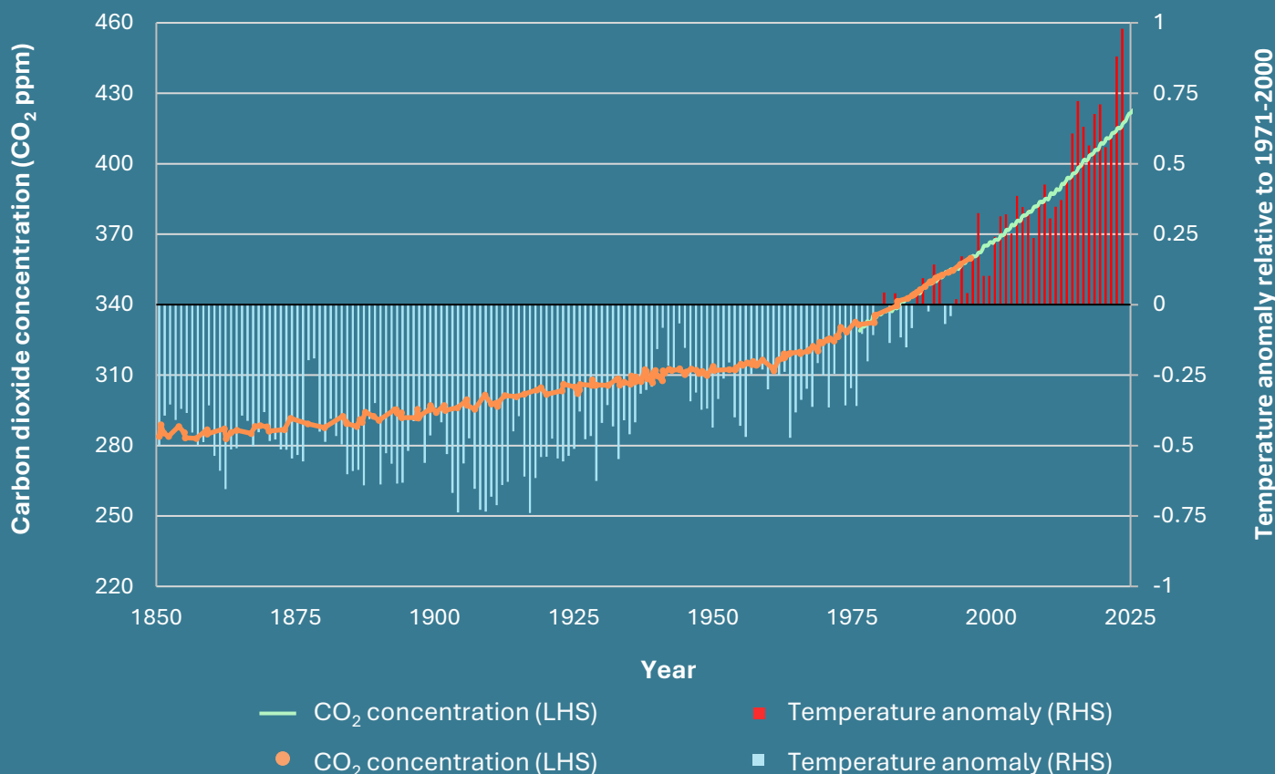
Figure 2: Carbon dioxide concentrations and temperature variations from 1850-2025
